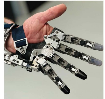
Partial Hand Robotics
